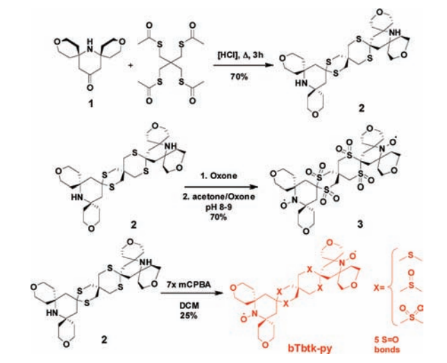
Scheme 1. Synthesis of bTbtk-py
